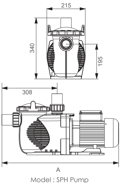
Model : SPH Pump
