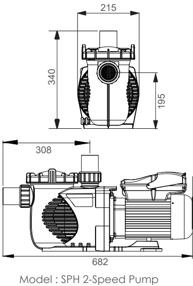
Model : SPH 2-Speed Pump
